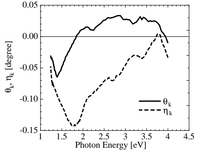
Fig. 4 Spectra of magneto-optical Kerr rotation (straight line) and Kerr ellipticity (dashed line) of the Mn-diffused layer measured at room temperature.
