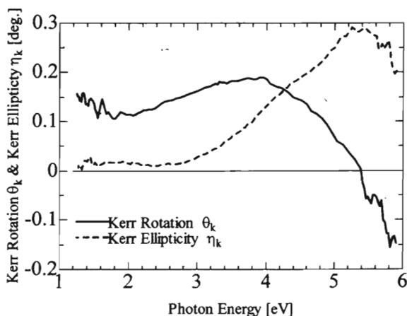
Fig. 2 Typical magneto-optical Kerr spectra of CoCrPt(50nm)/CoCrRu(50nm)/ \text{Al}_2\text{O}_3
