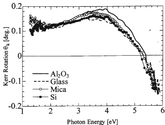
Fig. 3 Magneto-optical Kerr spectra of CoCrPt(50nm)/CoCrRu(50nm) on different substrates
