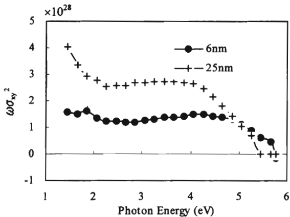
Fig. 9 Calculated \omega\sigma_{xy} of CoCrPt films with different thickness
