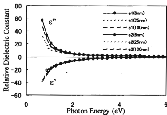
Fig. 8 Spectra of diagonal dielectric constant in \text{Co}_{71}\text{Cr}_{19}\text{Pt}_{10} films with different thickness values;
